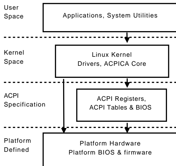
Figure 4: Platform Abstraction Layers
